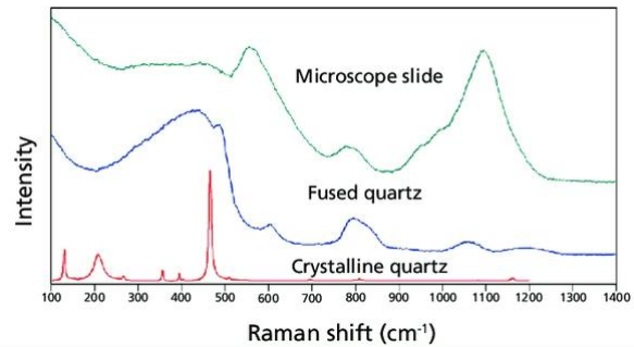
A comparison of glass vs crystalline equivalents based on Raman spectroscopy, from Tuschel (2017).
