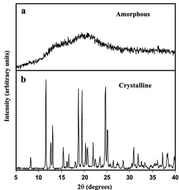
A comparison of the XRD spectra of glassy versus crystalline sucrose, from Nunes et al. (2005).
